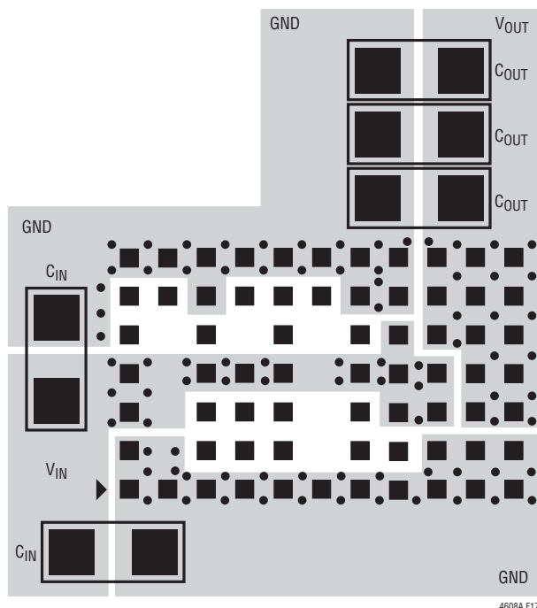
Figure 17. Recommended PCB Layout (LGA Shown, for BGA Use Circle Pads)
